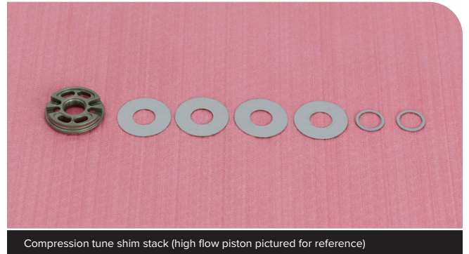
Compression tune shim stack (high flow piston pictured for reference)
