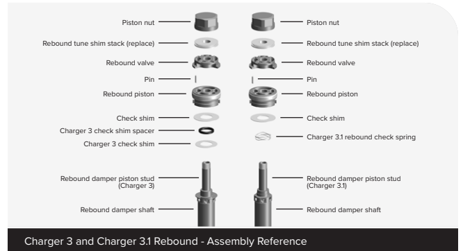
Charger 3 and Charger 3.1 Rebound - Assembly Reference
