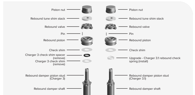
Charger 3 to Charger 3.1 - Rebound- Assembly Reference
